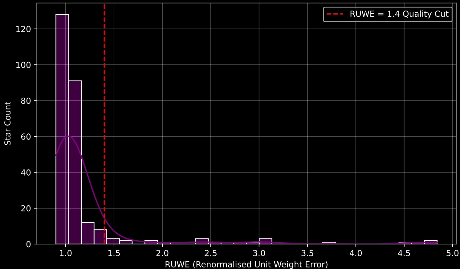
GALAH DR4 Field [1550] RUWE Distribution (n= 261)
